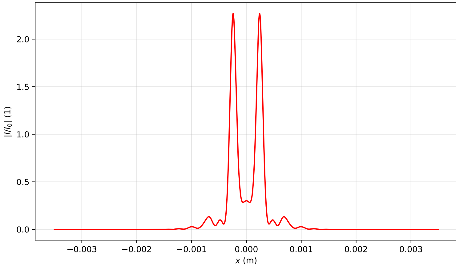
Intensity profile I(x, y = 0, z = 0.716)/I_0 , P_{in}=6.0P_{cr} , artificial time
